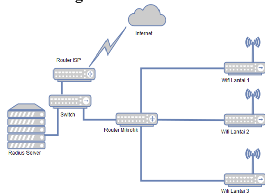
Gambar 4: Topologi Rancangan Prototype Jaringan Wifi
