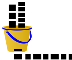
Gambar 1: Leaky Bucket
