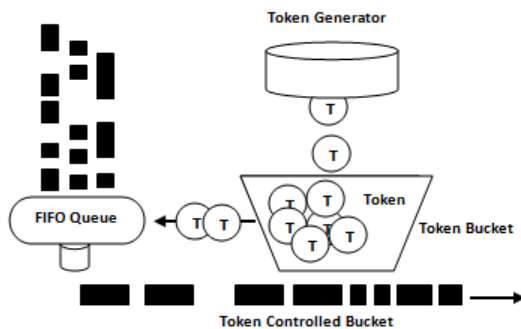
Gambar 2: Token Bucket
